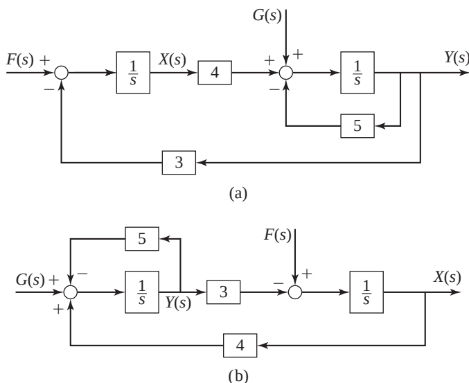
Figure 9.5.7 A diagram with two inputs.
