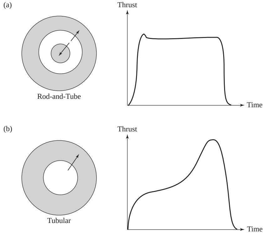
Figure 9.1.5 Solid fuel rocket thrust as a function of time.
