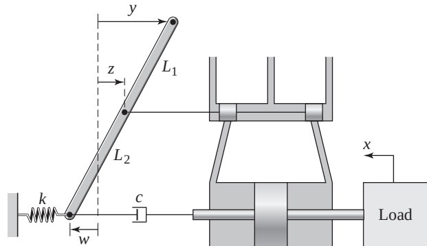
Figure 10.4.5 Hydraulic implementation of PI action.
