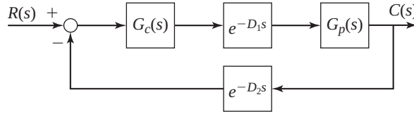
Figure 12.2.7 A system having dead-time elements in the forward path and in the feedback loop.
