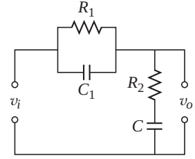
Figure 12.1.4 Passive lag-lead compensator circuit.
