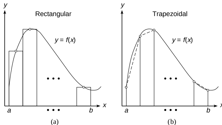
Figure D.1.3 Illustration of numerical integration by (a) the rectangular rule and (b) the trapezoidal rule.
