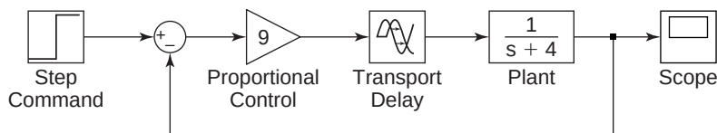
Figure 12.4.1 Simulink model using a Transport Delay block.
