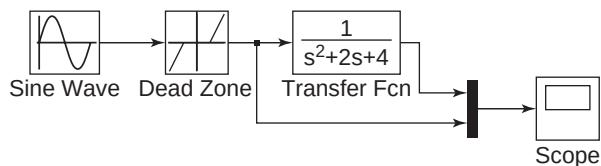
Figure 5.5.8 Modification of the dead-zone model to include a Mux block.
