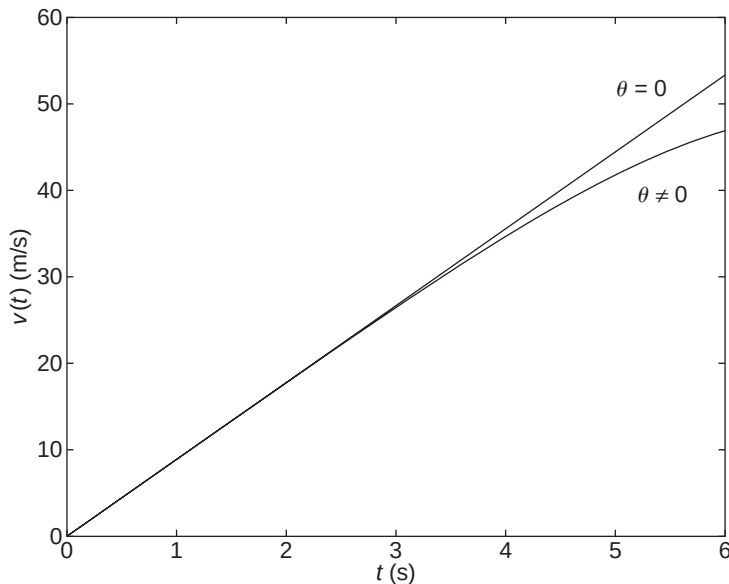
Figure 5.5.5 Speed response of the sled for \theta = 0 and \theta \neq 0 .
