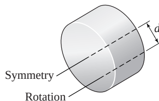
Figure 2.2.2 Illustration of the parallel-axis theorem.
