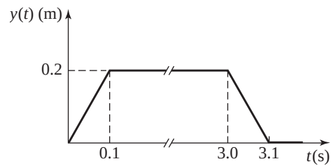
Figure 9.8.4 Bump profile.
