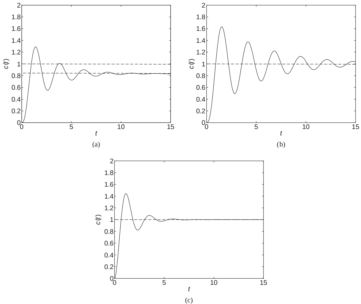
Figure 11.4.2 Unit-step responses of the controllers obtained in Example 11.4.1.
