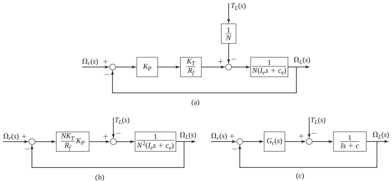
Figure 10.3.7 Model simplification for a speed control system with negligible field time constant.
