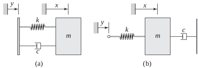
Figure 9.3.7 Effect of damper location on numerator dynamics.
