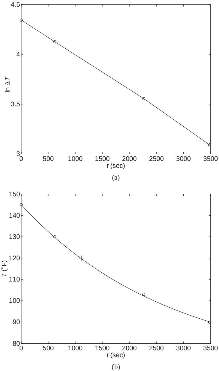
Figure 9.4.2 Temperature data. (a) Plot of transformed data. (b) Plot of the fitted equation.
