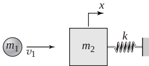
Figure 4.6.1 Inelastic collision.
