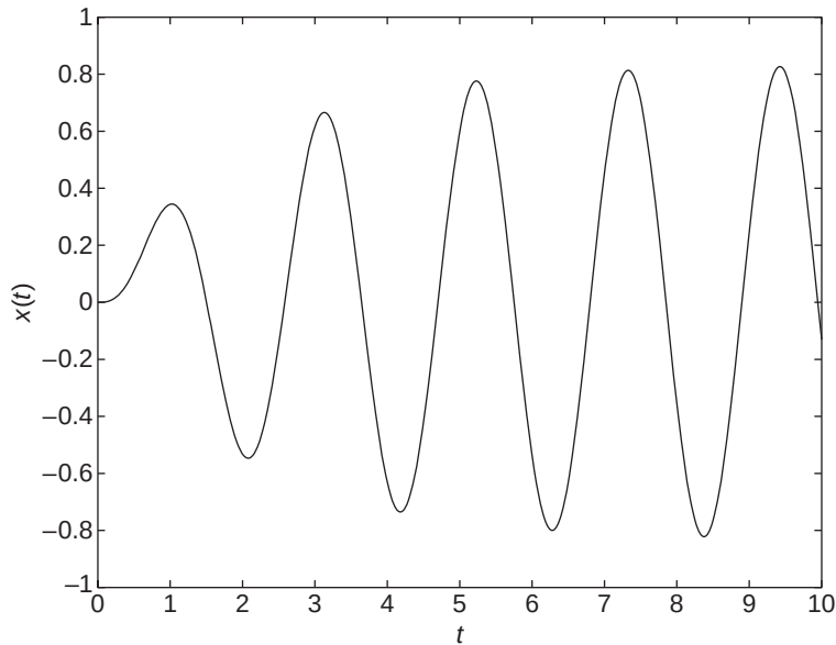
Figure 8.3.4 Response near resonance for a damped system.
