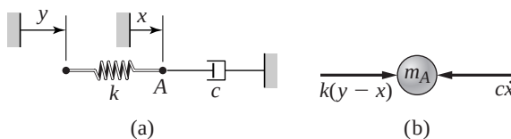
Figure 4.5.3 A system with negligible mass.
