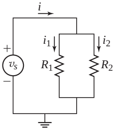
Figure 6.1.3 Parallel resistors.
