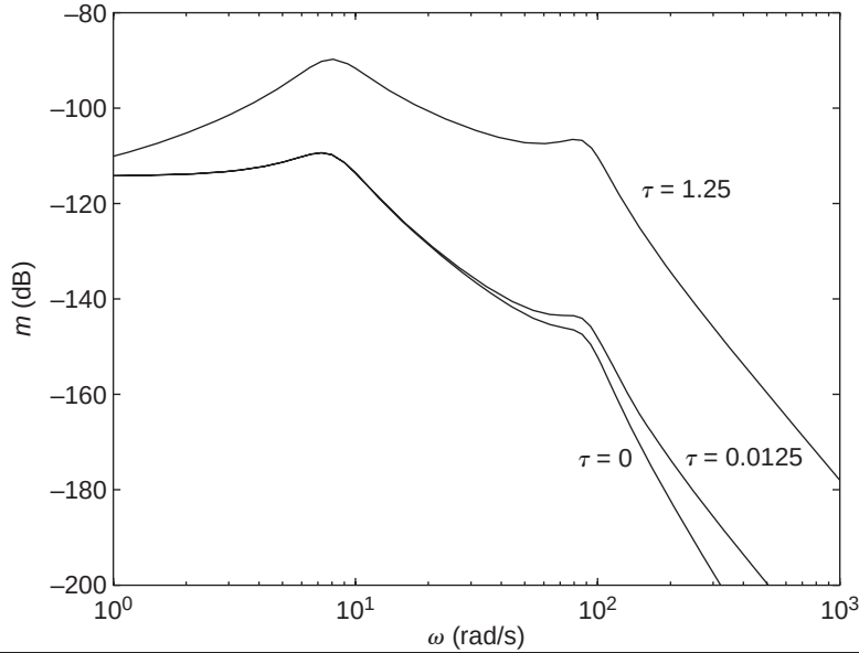
Figure 8.2.5 Log magnitude ratio plot of a fourth-order model.
