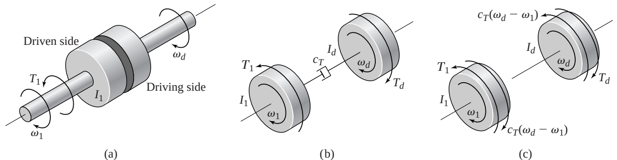
Figure 4.5.7 A two-inertia model of a fluid clutch.
