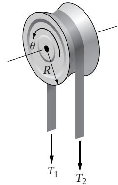
Figure 2.2.4 Pulley forces.
