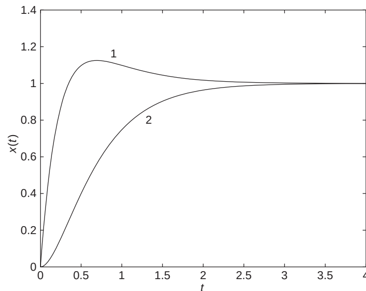
Figure 9.3.8 Response with and without numerator dynamics.
