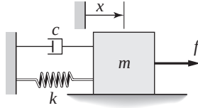
Figure 9.2.1 Some second-order systems.
