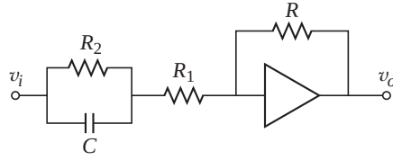
Figure 10.4.6 Op-amp implementation of PD action.
