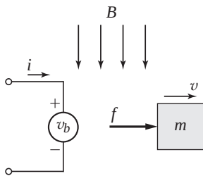
Figure 6.4.1 Electromagnetic interaction between electrical and mechanical subsystems.
