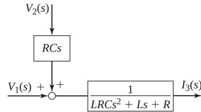
Figure 9.6.6 Block diagram of an RLC circuit with two voltage sources.
