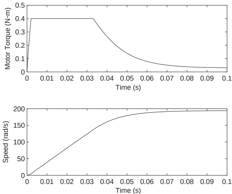
Figure 6.8.5 Response of a torque-limited motor.
