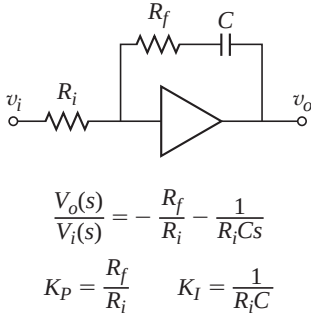
Figure 10.4.4 Op-amp implementation of PI action.
