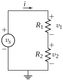
Figure 6.1.2 Series resistors.
