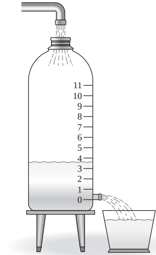
Figure 1.4.7 An experiment to determine flow rate versus liquid height.
