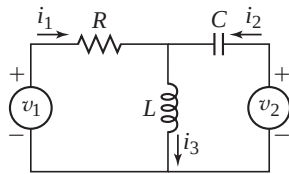
Figure 9.6.5 An RLC circuit with two voltage sources.
