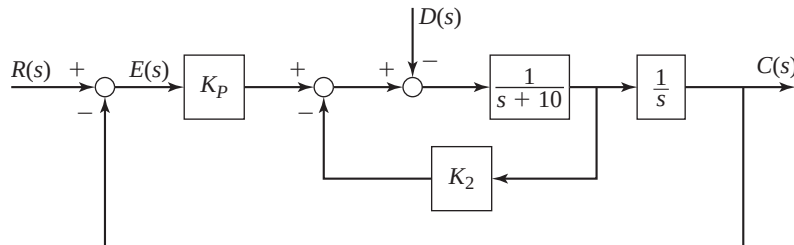
Figure 10.8.2 P action with internal feedback.
