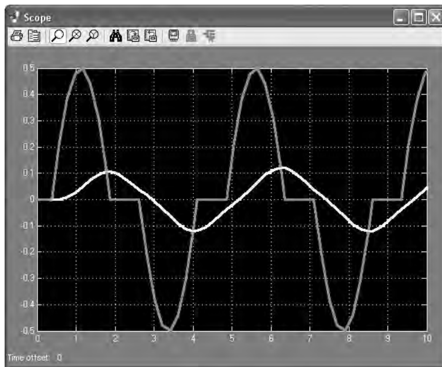
Figure 5.5.9 The response of the dead-zone model.
