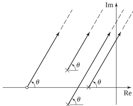
Figure 11.2.6 Illustration of guide 6.
