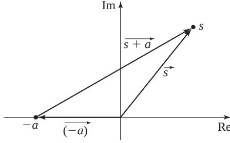
Figure 11.2.3 Vector addition and vector representation of complex numbers.
