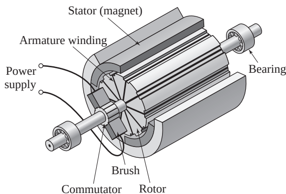
Figure 6.4.3 Cutaway view of a permanent magnet motor.
