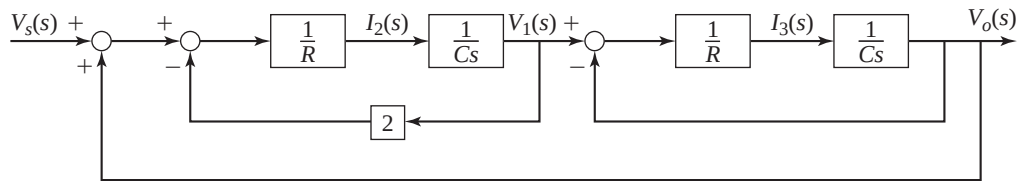
Figure 9.6.8 Block diagrams of coupled RC loops.
