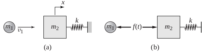
Figure 4.6.3 Perfectly elastic collision.
