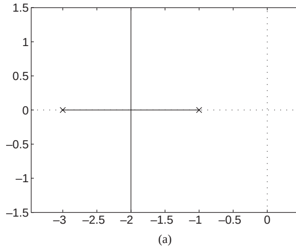
Figure 11.2.8 Root locus plots for some second-order equations.
