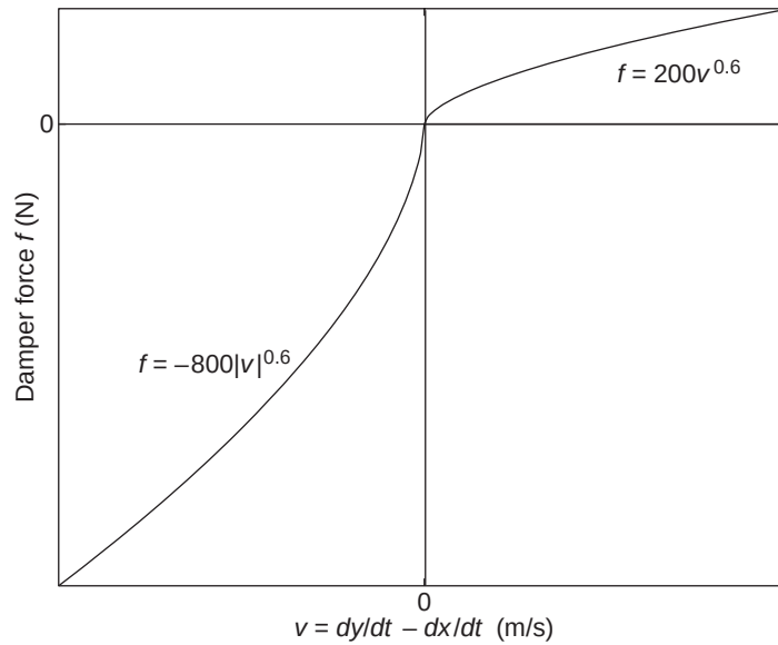
Figure 9.8.3 Degressive damper model.
