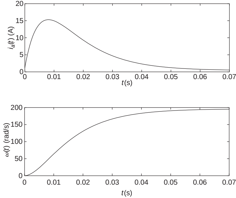
Figure 6.5.1 Step response of an armature-controlled dc motor.
