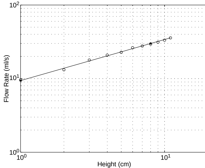
Figure 1.4.9 Log-log plot of flow rate data.
